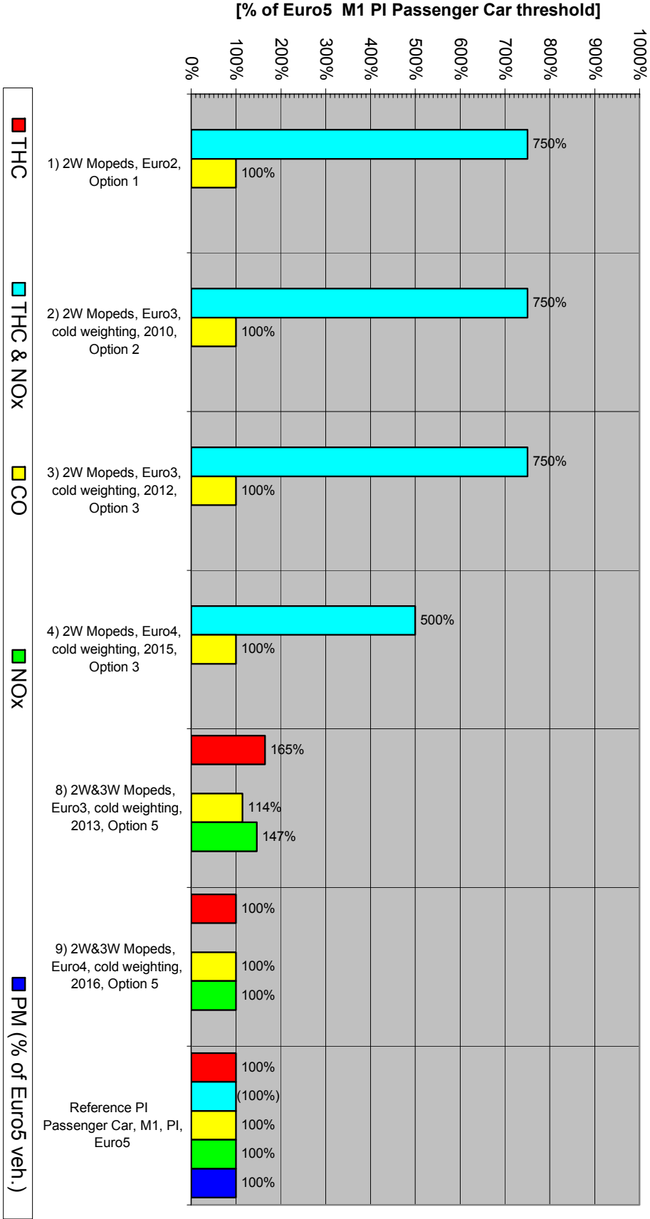
Figure 11: Overview current, proposed and bench mark emission limits for 2 wheel Mopeds (classes L1e)
