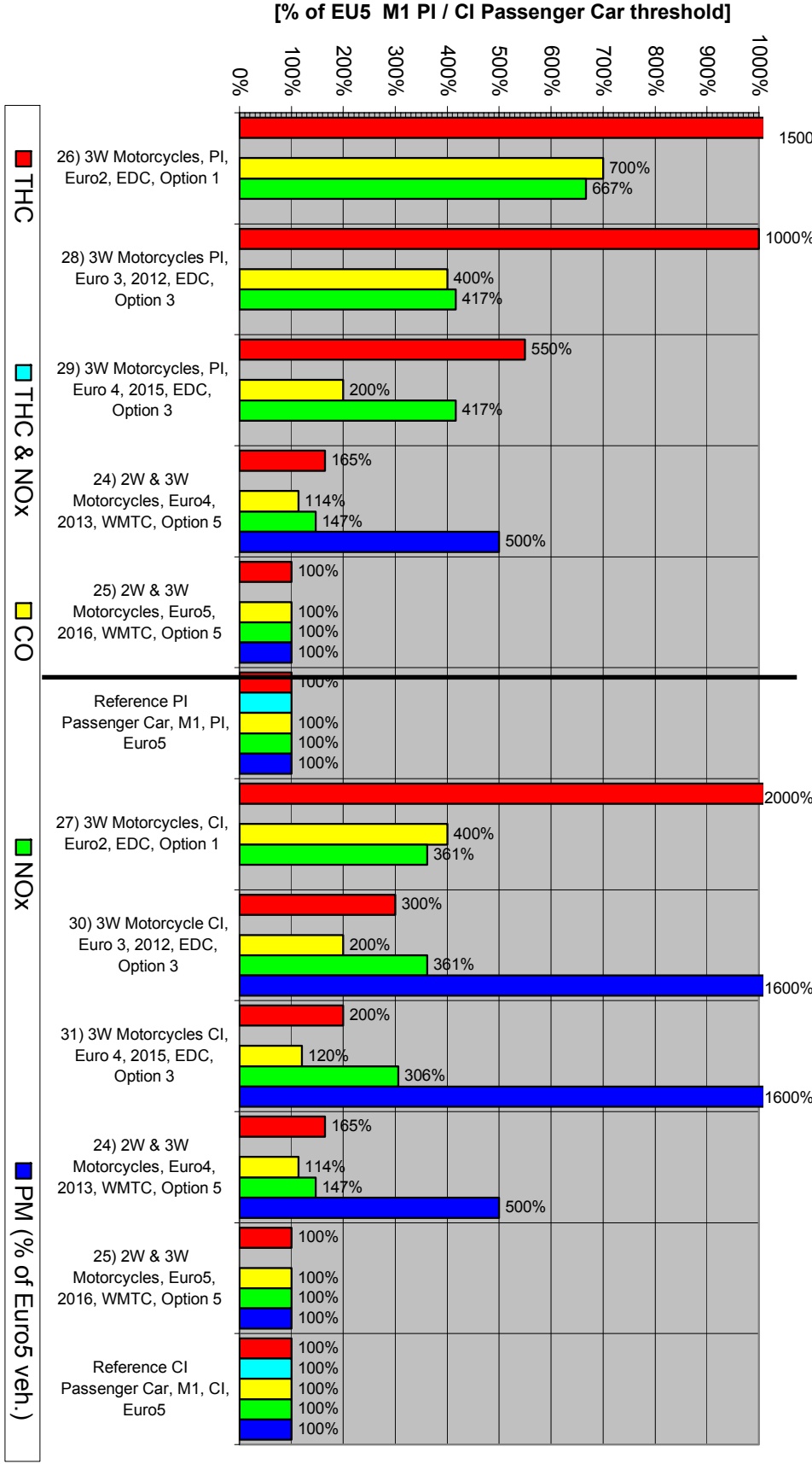
Class L5, 3-wheel Motorcycle (Tricycle), overview current and proposed limits [% of EU5 M1 PI / CI Passenger Car threshold]
