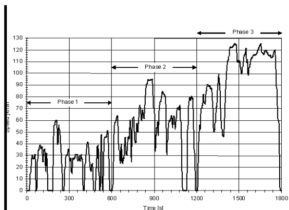
WMTC alternative driving cycle for the type-approval of Euro3 L3e motorcycles
