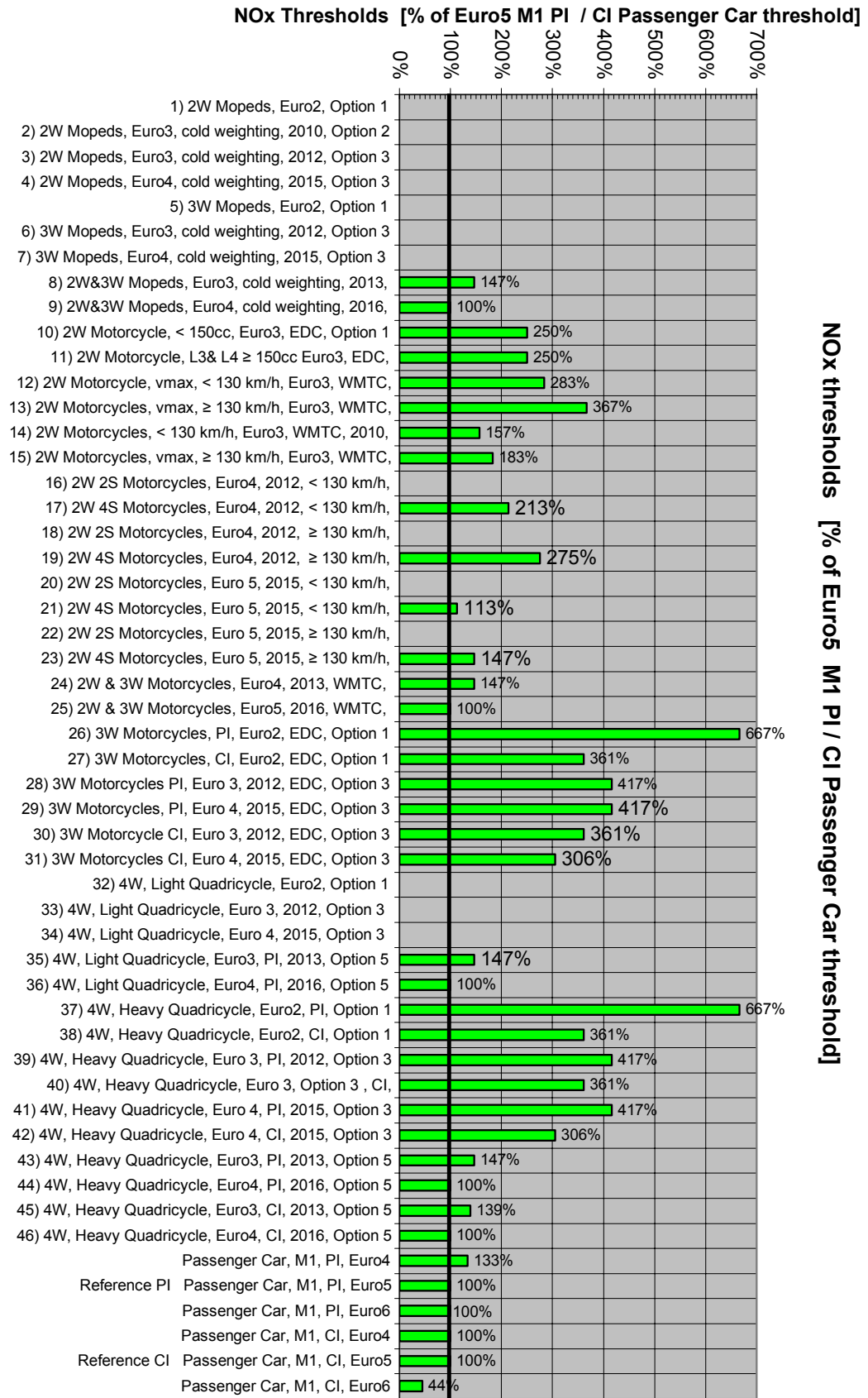
Figure 20: Overview current, proposed emission limits for all L-category vehicle categories vs. passenger car M1 benchmark limits: Nitrogen Oxides (NOx)
